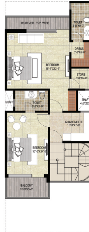
FIRST FLOOR PLAN C.A. = 880.00 sqft.
